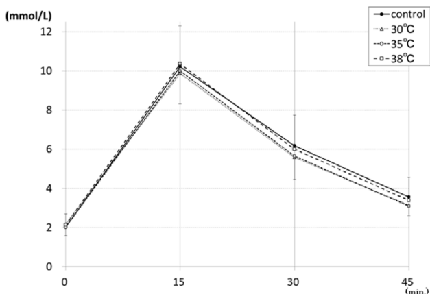
Fig.1. Time course of Plasma lactate concentrations of control, 38°C, 35°C and 30°C immersion. Values are means ± SD.
