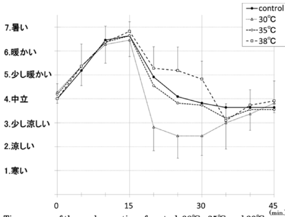
Fig.8. Time course of thermal sensation of control, 38°C , 35°C and 30°C immersion. Values are means±SD.
