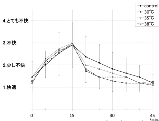
Fig.9. Time course of comfort sensation of control, 38°C , 35°C and 30°C immersion. Values are means±SD.
